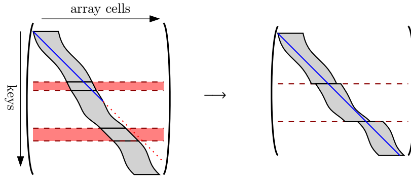
an overloaded data structure where not all keys could be placed
