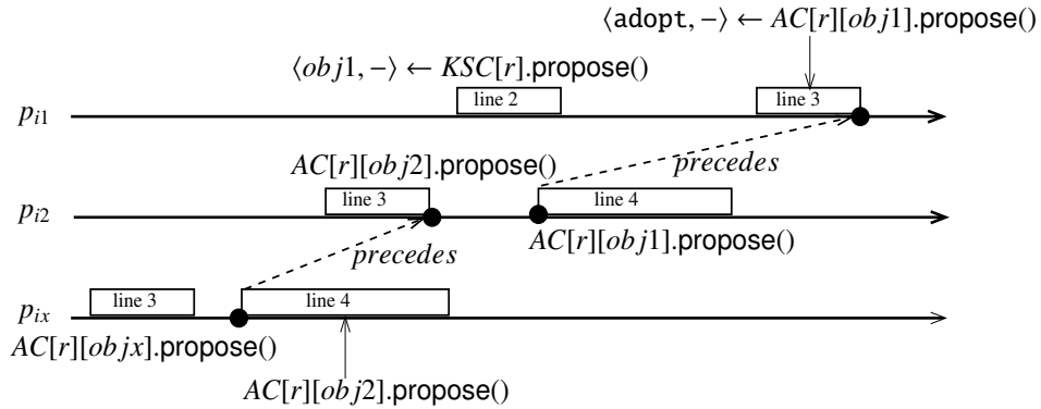
Figure 9: Net effect of the k -SC and CA objects used at lines 2-4 of round r
