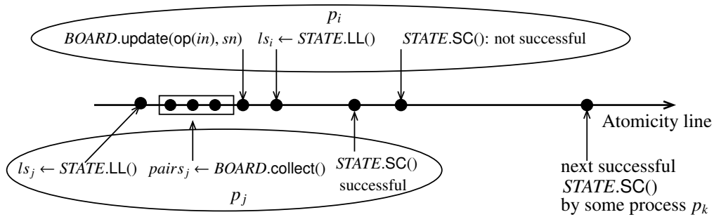
Figure 4: Why to repeat twice lines 4-12 (big dot = atomic step)
